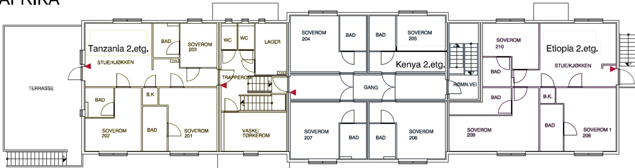
PLAN 2
