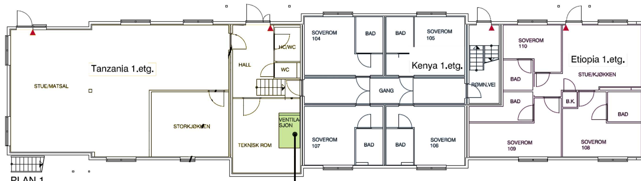
PLAN 1
